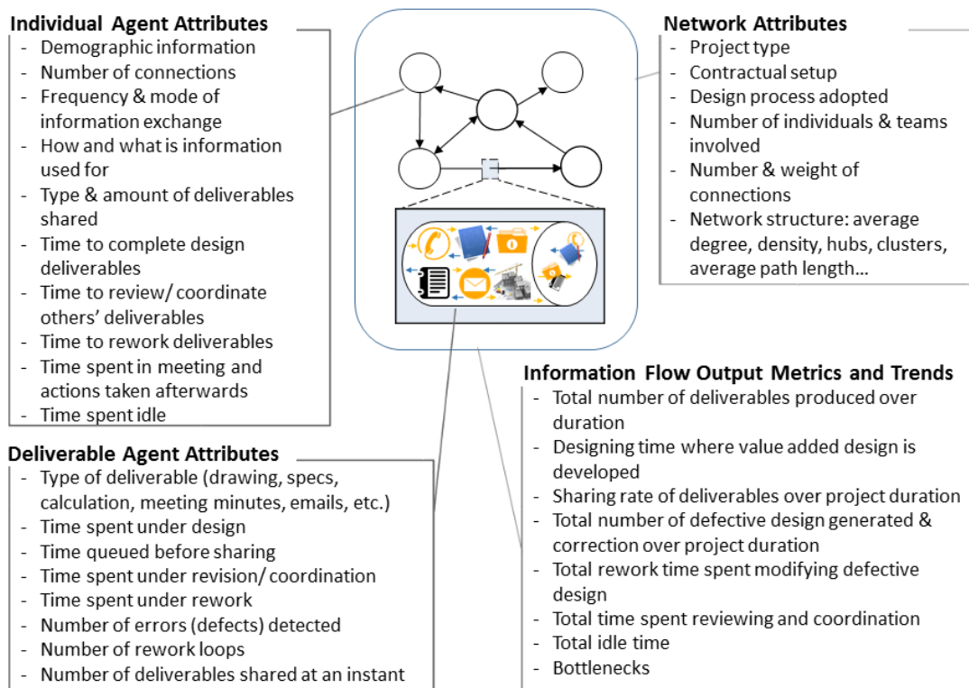
Figure 2. Social network topology, agents' attributes, and output metrics
