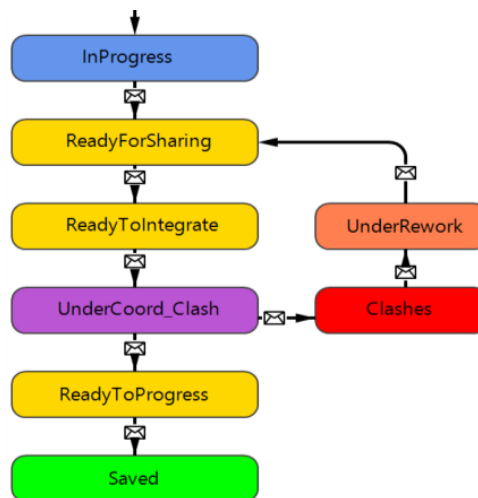
Figure 4. BIM model state chart
