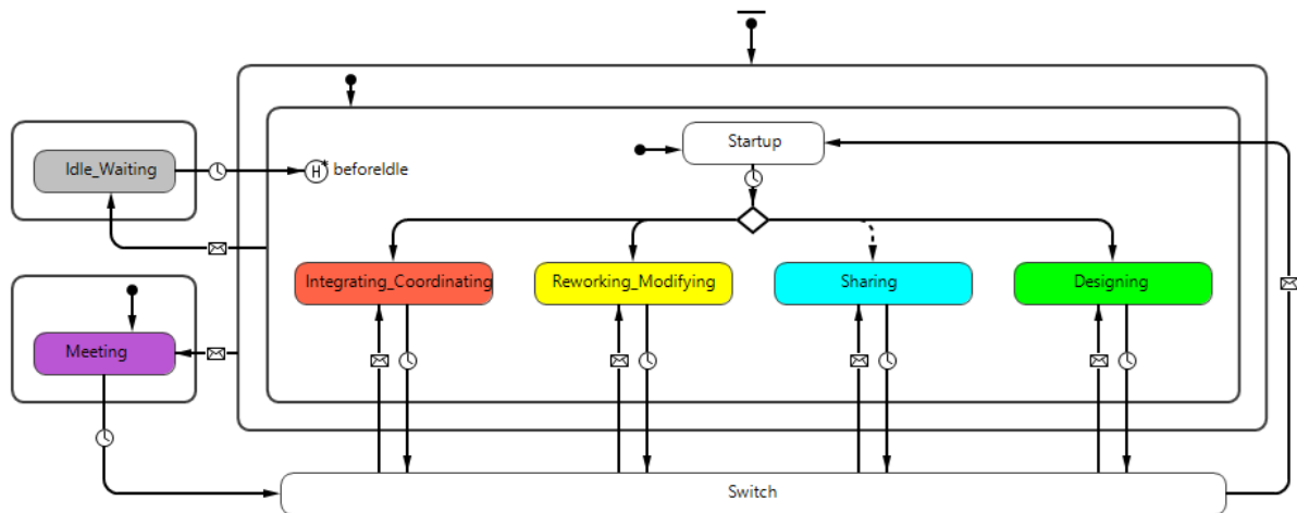
Figure 3. Designer state chart of behaviours
