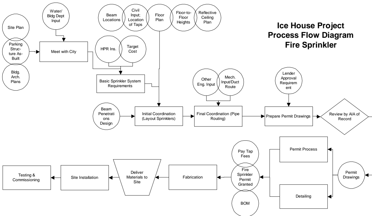
Fire Sprinkler Process Flow Diagram
