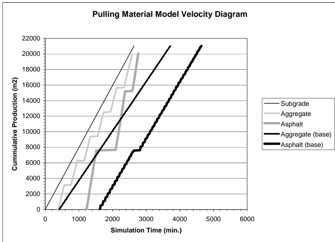
Fig. 9. Pulling material base model - velocity diagram (med. haul, 30-kms)
